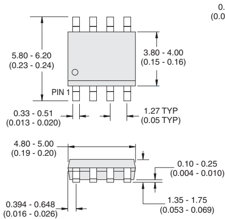
8-Pin SOIC Package
