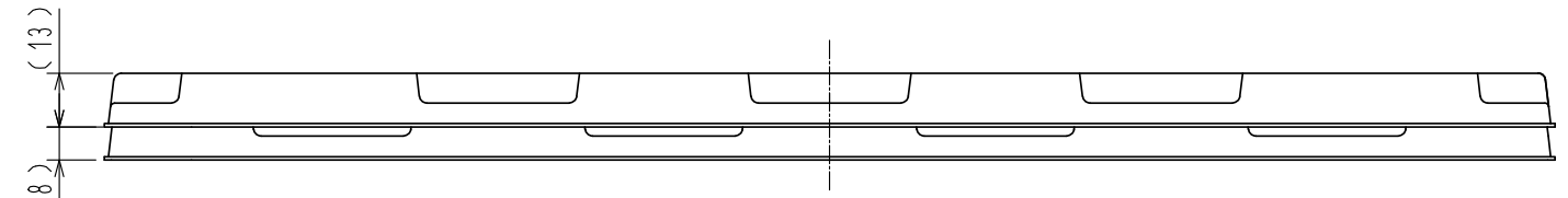
Fig.4 Stacked tray drawing (1:2)
